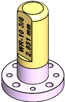
WR-10 WAVEGUIDE OFFSET
